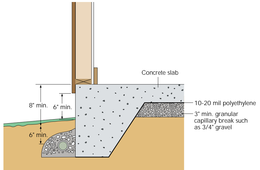
FIGURE 2 SLAB-ON-GRADE FOUNDATION
